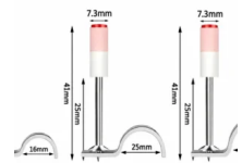
Pipe Clip Pin Nails for Nail Guns – 16mm, 25mm &amp; 32mm
